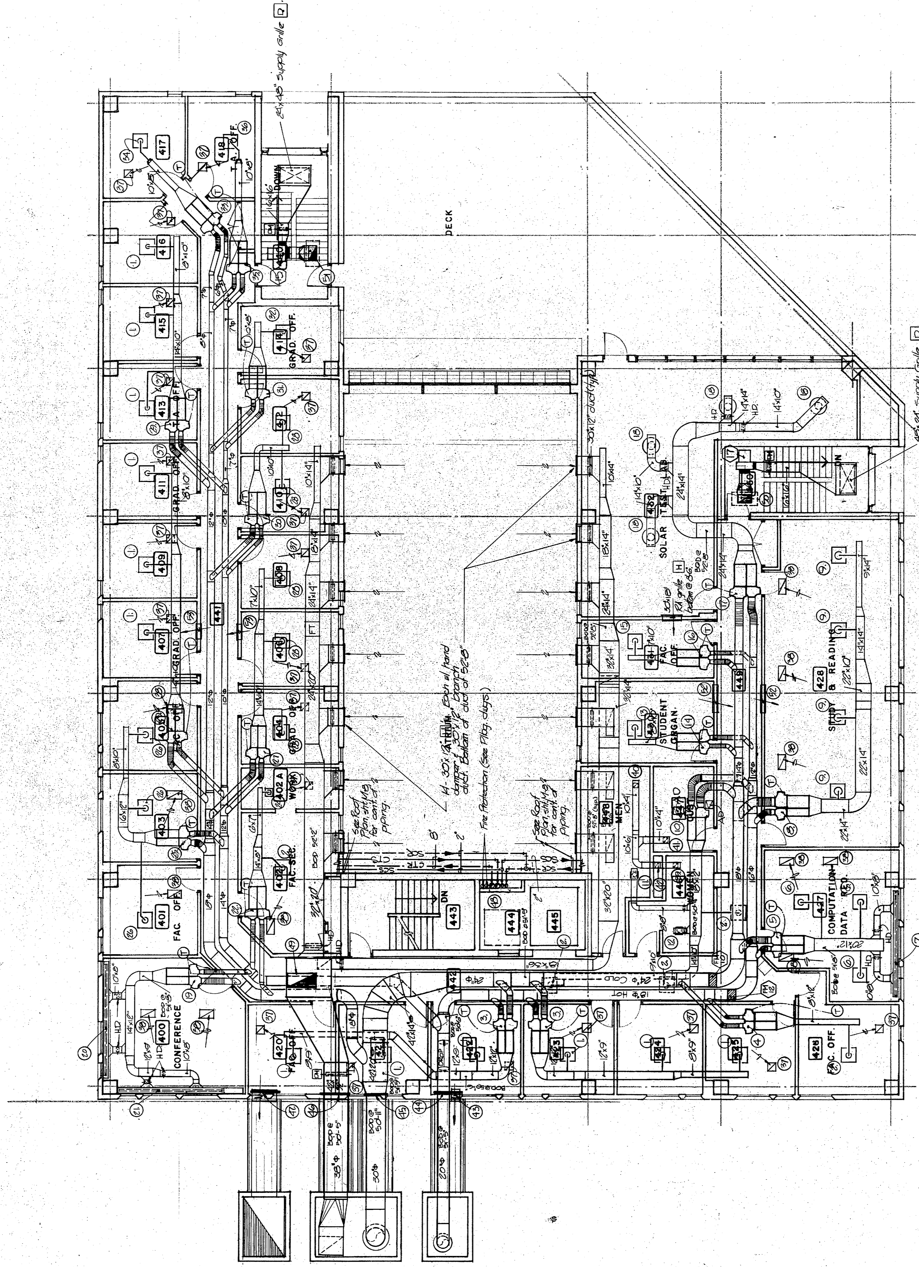
NORTH FLOOR PLAN, LEVEL 4 1/8" = 1'-0"
